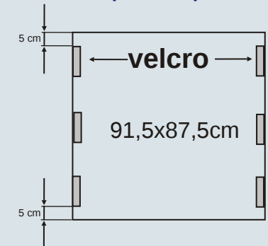
VarioDesk 1B Graphic panel
